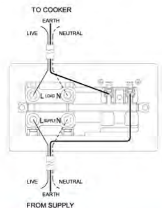
COOKER CONTROL UNIT
